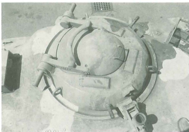
Israeli dissatisfaction with the M1 commander's cupola led to the development of a low-profile cupola similar to that first employed on the M48, but without the external machine gun cradle assembly. This has been manufactured by Urdan and is used on Israeli, American and some exported Pattons. (George Balin)
