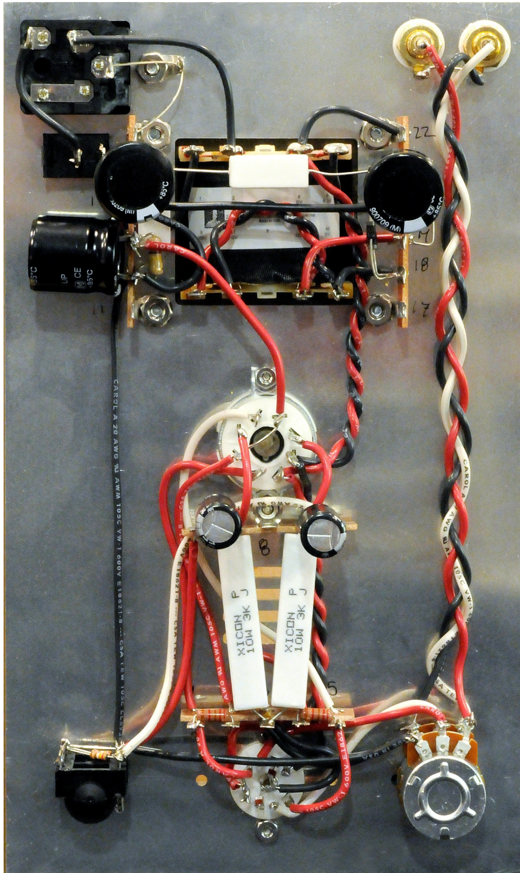
The completed Crack output transformerless tube headphone amplifier
